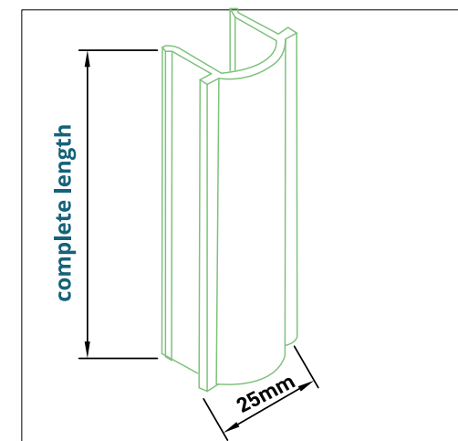
ALMN - COVERING PROFILE
