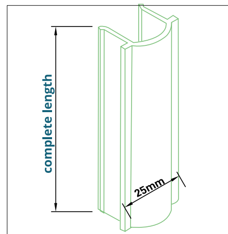
ALMN - COVERING PROFILE
